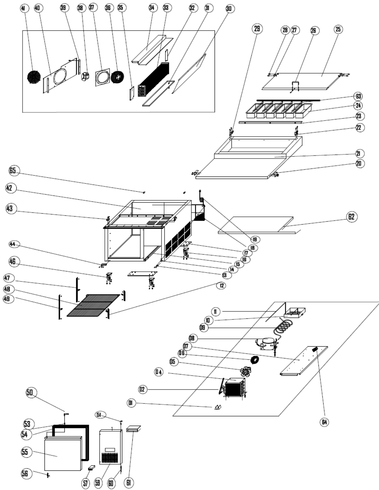
EXPLODE OF KCHPT50.6
